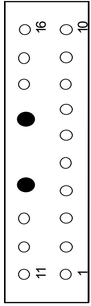
Connector Layout (front view)
